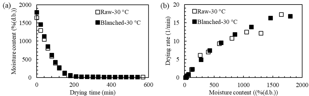
Fig. 1 Drying curve of each sample at an air velocity of 3 m/s and a temperature of 30 °C (a) Changes in moisture content; (b) drying characteristics curves
