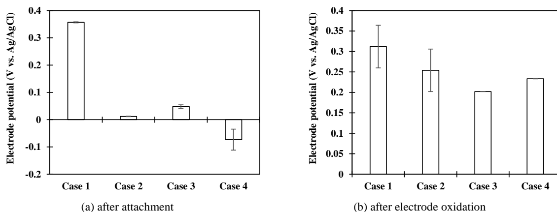
Fig. 3 Comparison of electrode potential at different conditions
