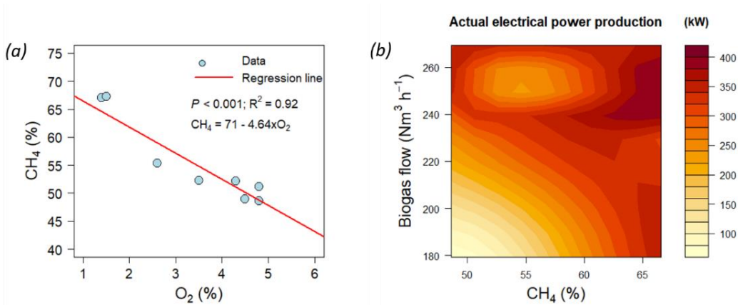
Fig. 3 Relationship between CH 4 and O 2 (a) & Determination of average load as a function of biogas flow and CH 4 (b)
