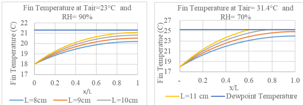
Fig. 1. Fin temperature distribution of different fin lengths at (a) T_a = 23^\circ C and RH = 90\% , (b) T_a = 31.4^\circ C and RH = 70\% .
