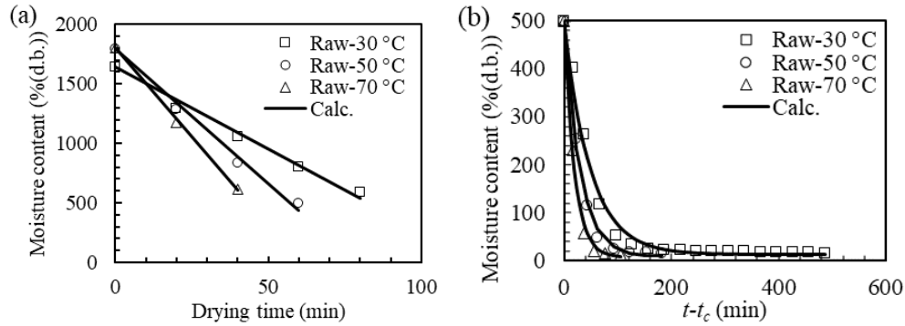
Fig. 2 Comparisons of observed moisture content changes with the results calculated from (a): Eq. (1) and (b): Eq. (2) at an air velocity of 3 m/s for the raw sample during drying
