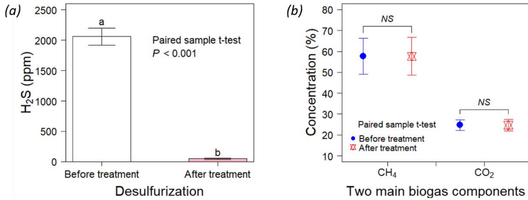
Fig. 2 Comparison of H 2 S (a) & CH 4 and CO 2 (b) before and after desulfurization (Mean \pm SD; N = 21). Paired sample t-test was used for the analysis. Different alphabetic letters denote significant differences at the error level of 0.05, and NS means non-significance.
