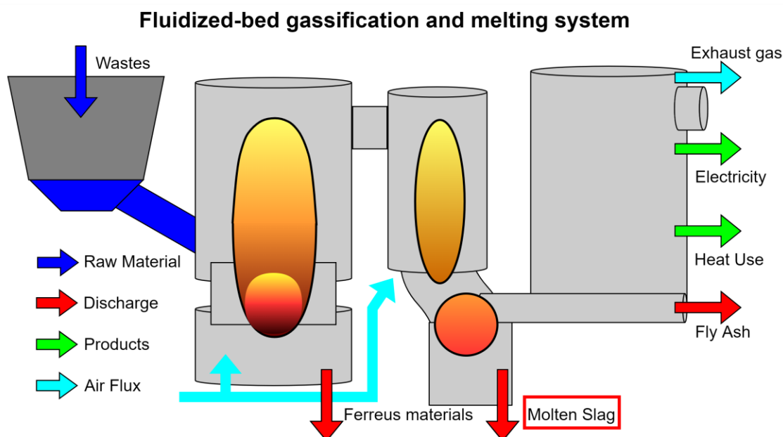
Fig. 5 Municipal Solid Waste Incineration process
