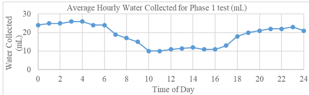
Fig. 5 Average Hourly Water Collection for the AWG Device
