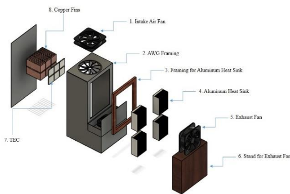
Fig. 3 Blow up picture of the AWG Device with its corresponding parts (a) and finished product and experimental setup (b).
