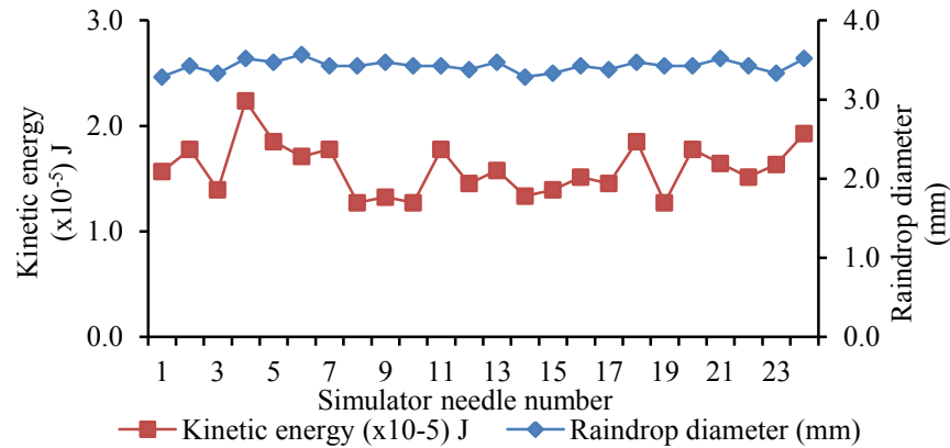
Fig. 3 Kinetic Energy and raindrop diameter
