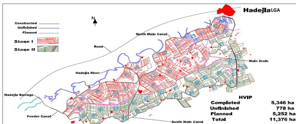
Fig. 1 Layout of Hadejia Valley Irrigation Project (HVIP) phase I (stages I and II)
