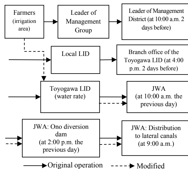
Fig. 3 The original and modified water allocation method and distribution process in Toyogawa irrigation project
