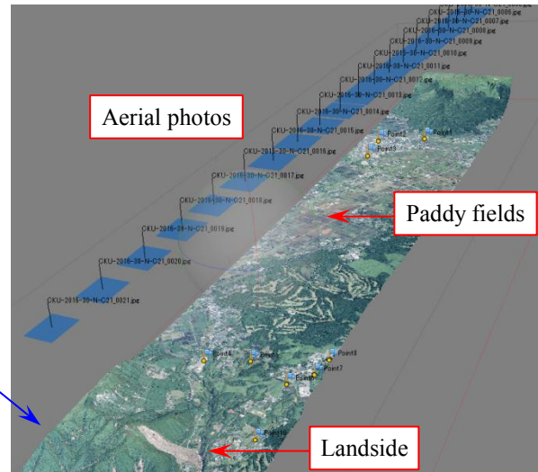
Fig. 2 The 3D model by aerial photogrammetry
