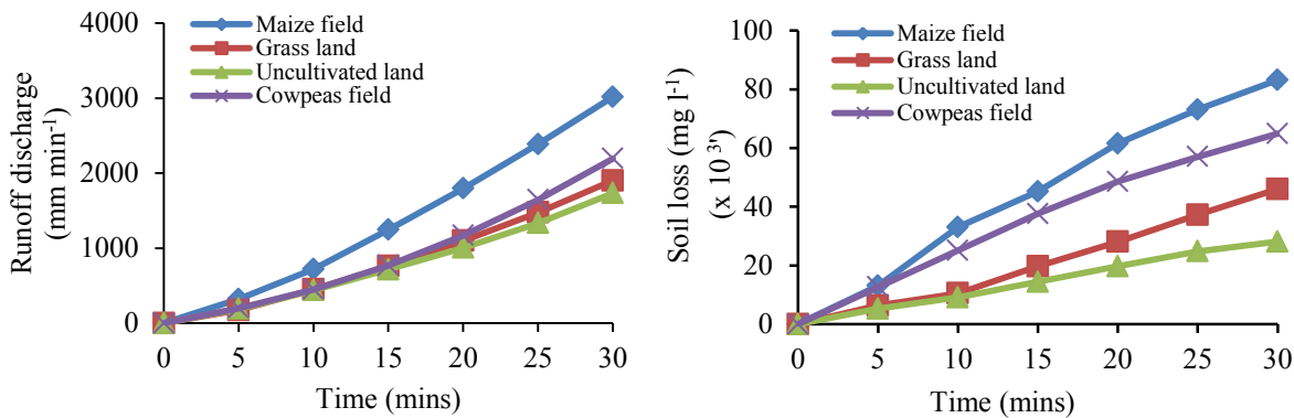
Fig. 6 Runoff discharge and soil loss graphs for different soil field types
