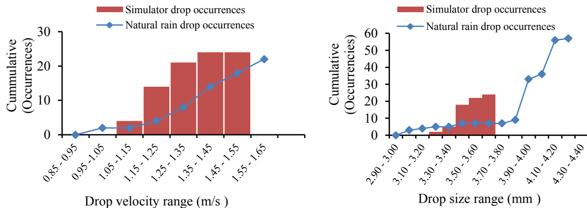
Fig. 5 Natural rain drop and simulator drop relation on drop velocity and drop size
