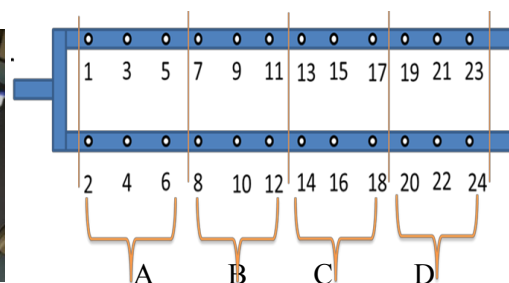
Fig. 1 Materials for artificial portable rainfall simulator Fig. 2 Needles numbering and grouping
