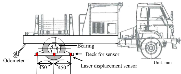
Fig. 2 Sensor configuration
